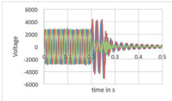
Figure 5 Motor terminal voltages during a simulated earth fault on the motor
