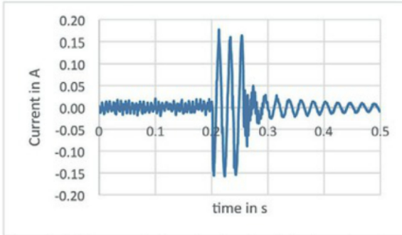
Figure 4 Fault current during a simulated earth fault on the motor terminal
