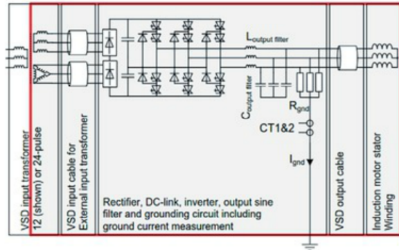
Figure 1 Protective zone for power drive systems
