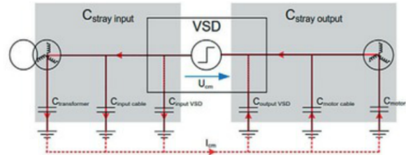
Figure 3 Zero-sequence diagram
