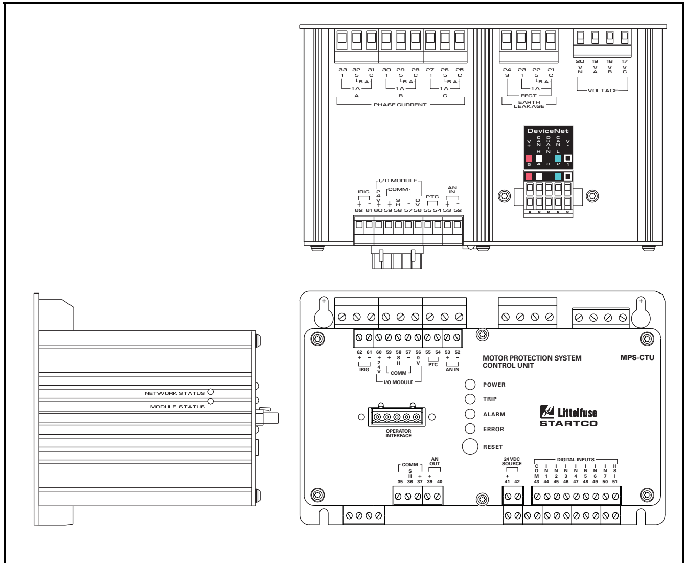
FIGURE 1. Outline Drawing.
